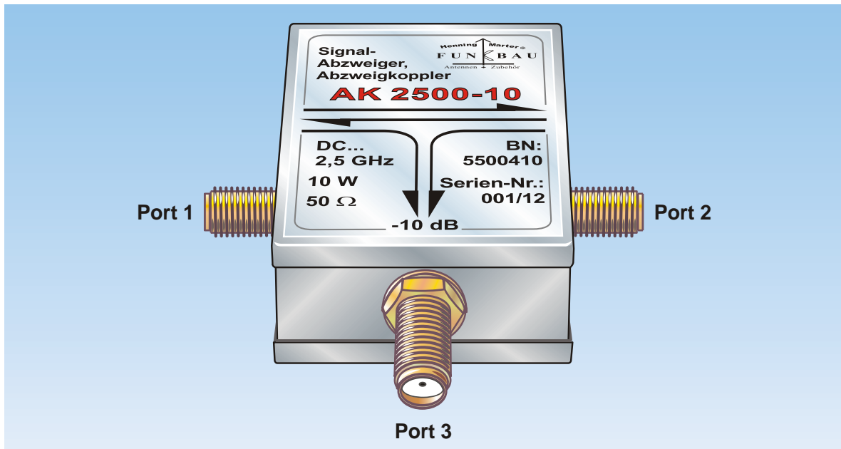
Ansichten/Abmessungen (Views/Dimensions)
