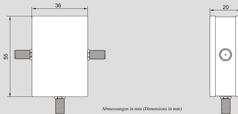
Ansichten/Abmessungen (Views/Dimensions)
